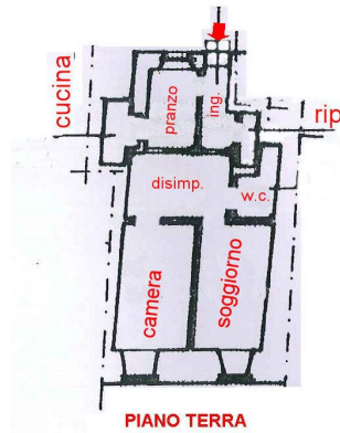
PIANO TERRA
